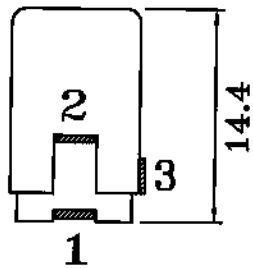
TERMINAL NUMBERS
