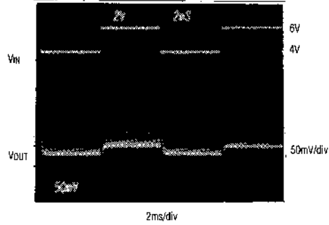
LINE-TRANSIENT RESPONSE
