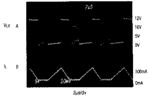
SWITCHING WAVEFORMS - DISCONTINUOUS CONDUCTION
